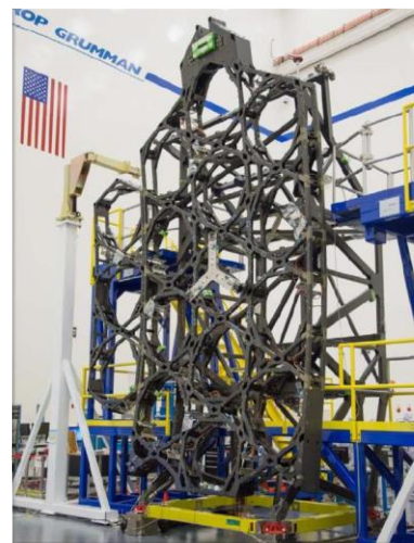
Flight telescope backplane & with one wing installed
