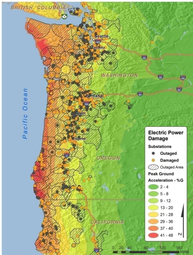
Electric power infrastructure damaged and outaged
