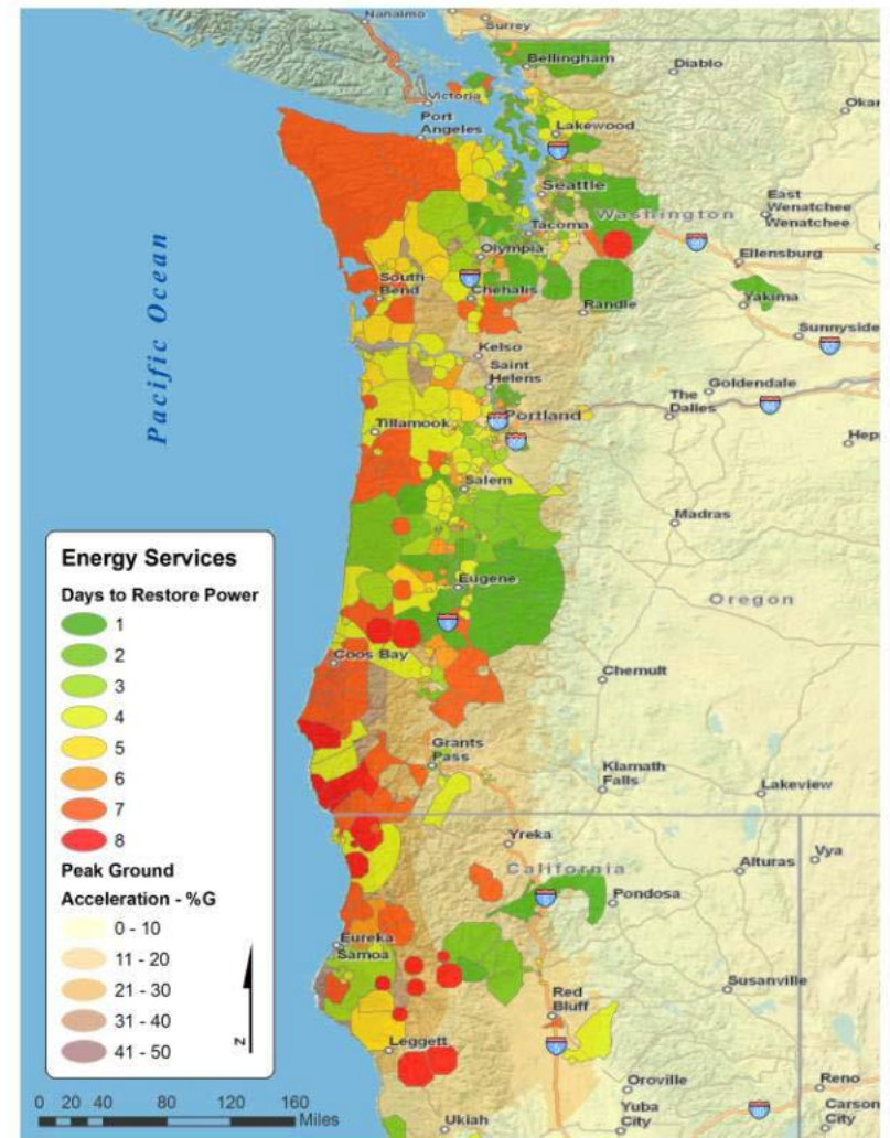
Estimated restoration times for damaged and outaged substations
