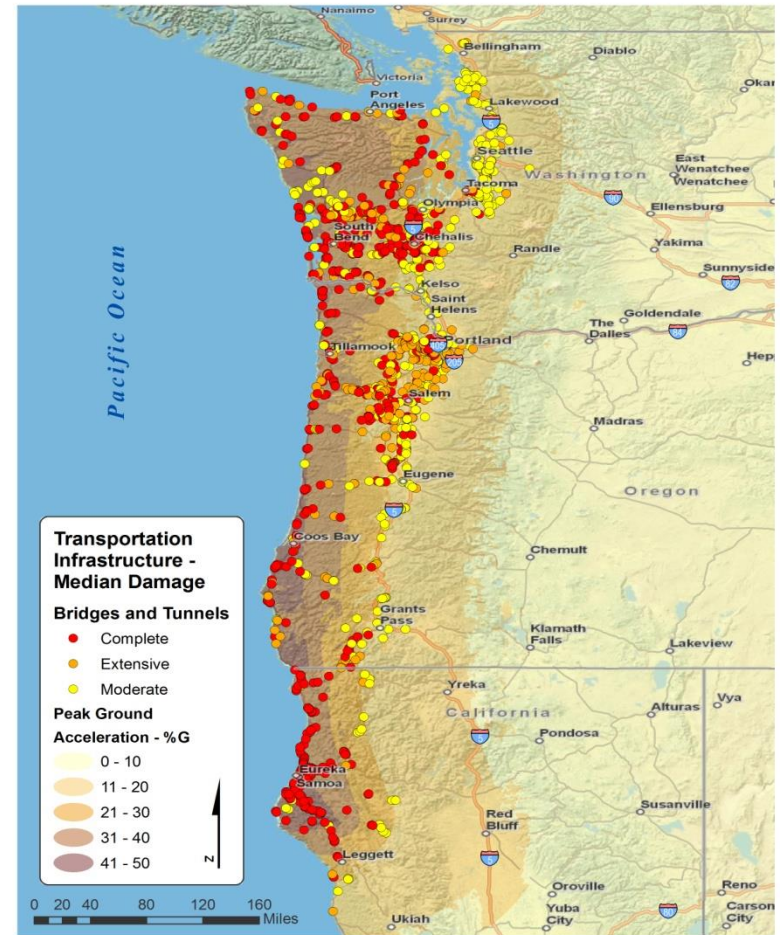
Expected damage to highway bridges and tunnels in the Cascadia region
