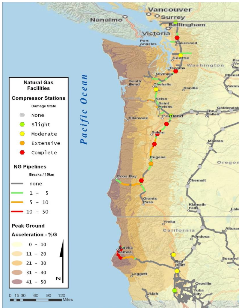
Estimated damage to natural gas pipelines and compressor stations
