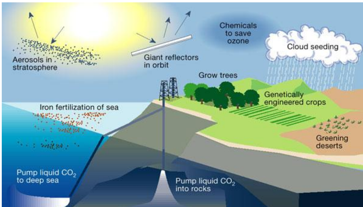
A schematic representation of various geoengineering and carbon storage proposals (courtesy B. Matthews). Source: http://pesd.stanford.edu/news/science_progress_geoengineering/# .
