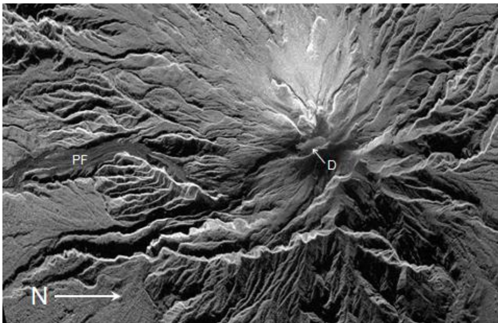
TerraSAR-X Synthetic Aperture Radar image of 4 Nov 2010, showing pyroclastic flow deposits (PF) from the 26 October eruption and a new lava dome that growing at the summit. Very rapid growth of the lava dome was followed by a large eruption during the night of 4-5 November.
