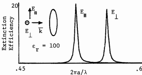
Fig. 1: Resonances of a dielectric prolate spheroid. Major semi-axis = \underline{a} . Minor semi-axis = \underline{b} .
