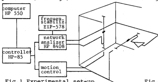
Fig.1 Experimental set-up
