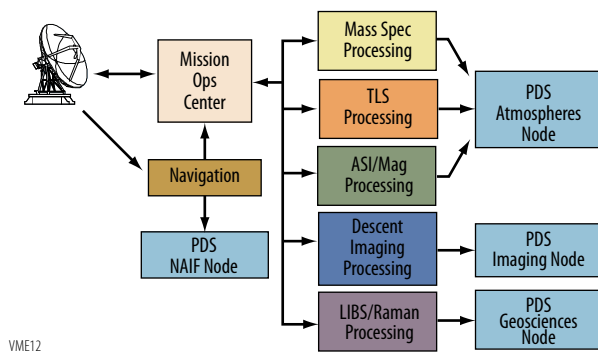
Figure 14: Ground System Block Diagram
