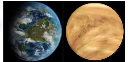
Left: Artist's rendition of early Venus with possible large oceans and a significant hydrologic cycle; Right: Venus today with a dry, thick CO 2 greenhouse atmosphere resulting in surface temperatures of 450°C and pressures in excess of 90 bar.
