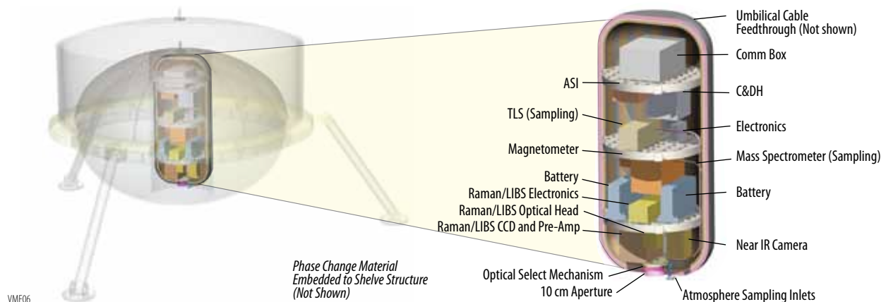
Figure 7: Lander with gondola details, showing instruments and avionics.
